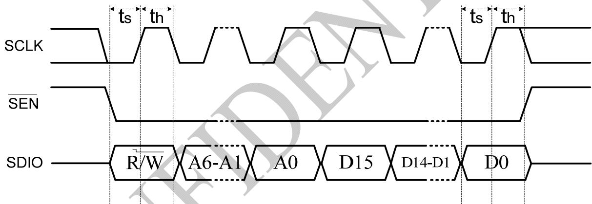
Figure5. Three-wire Interface Write Timing Diagram
